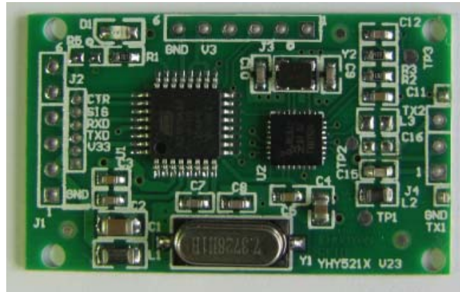
Figure 5– YHY521X top view
