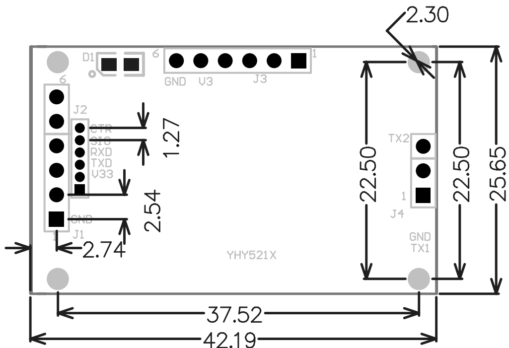
Figure 3– YHY521X Top view size
